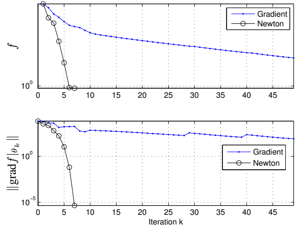
Fig. 5. Intrinsic gradient and Newton algorithms: performance evaluation. Value of the cost function f (top) and norm of the intrinsic gradient \|\text{grad} f|_{\theta_k}\| (bottom).
