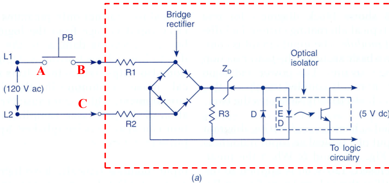
Electronic circuit
