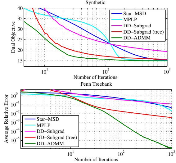
Figure 4. Dependency parsing with 2nd-order models. For DD-subgradient, we consider both tree-based and flow-based factor graphs, and \eta_0 as in Fig. 1. DD-ADMM ( \eta = 0.05 , \tau = 1.5 ), MPLP, and Star-MSD ran only on the flow-based factor graph (see footnote 2). DD-Acc is not shown due to numerical problems when computing some low-temperature marginals. Top: synthetic 10-word sentences; we randomly generated (unary) arc log-potentials from N(0, 1) and (pairwise) grandparent and sibling log-potentials from N(0, 0.1) . Bottom: §23 of the Penn Treebank; the plot shows relative errors per iteration w.r.t. the dual optimum, averaged over the 2,399 test sentences.
